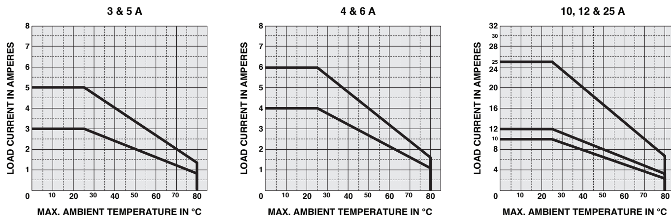
Load Current vs Ambient Temperature (100% Duty Cycle)
