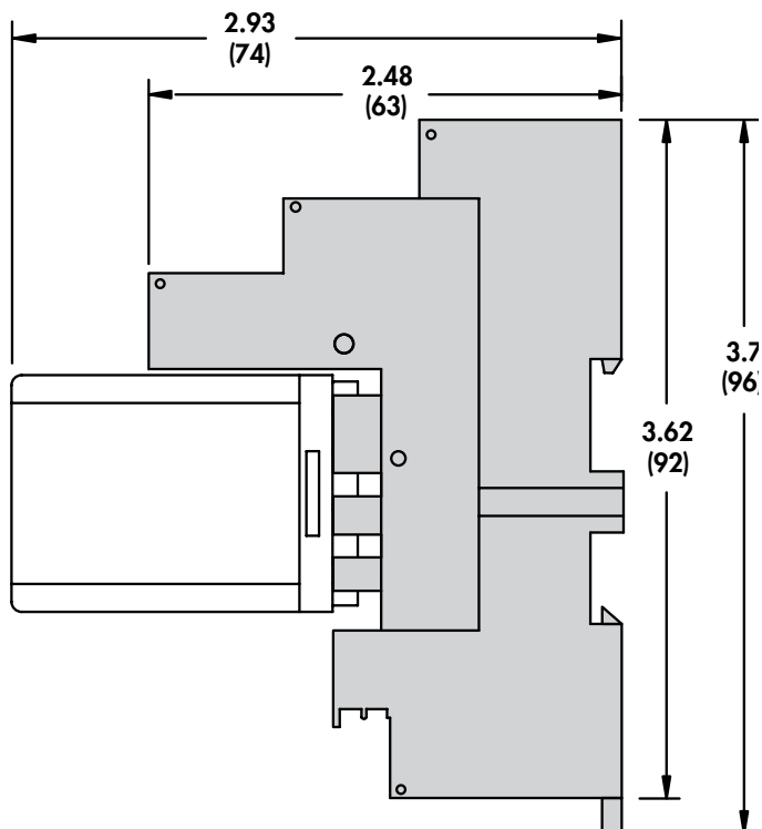
70-788EL11-1 SOCKET
