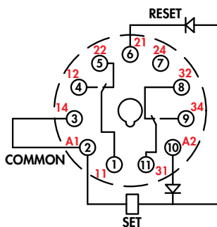
Single Coil (AC)
