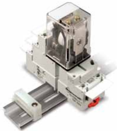
755 Relay with the 70-750EL11-1 Socket
