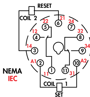
Dual Coil (DC)
