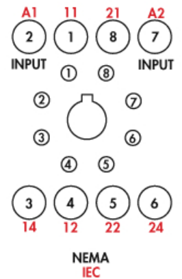
Wiring Diagram Top View
