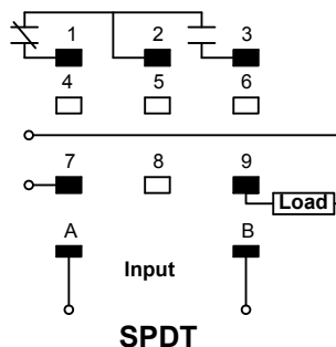
235 Wire Diagram
